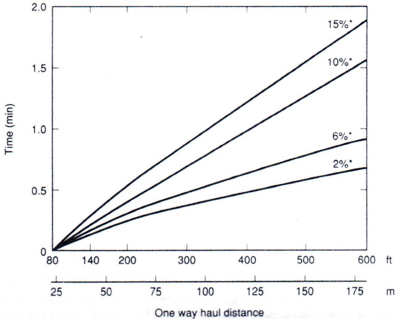
FIGURE 4-15: Travel time, wheel loader ( haul + return ).
