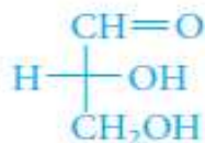
Fischer projection
