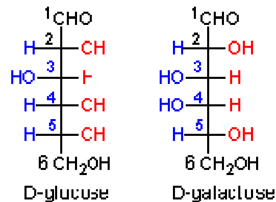
Diastereomers
