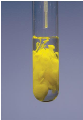
\text{PbI}_2
