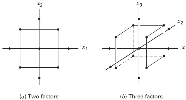
■ FIGURE 6.39 Central composite designs
