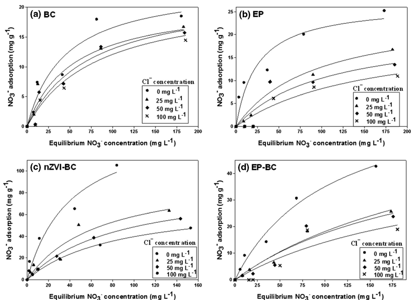
Fig. 7 Nitrate sorption onto a date palm tree leaf biochar (BC), b eggshell powder (EP), c nano zerovalent iron-composited BC (nZVI-BC), and d EP-composited BC (EP-BC) as influenced by the presence of various chloride ion concentrations in the aqueous media (0, 25, 50, and 100 \text{mg Cl}^- \text{L}^{-1} )
