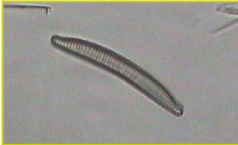
Diatoms sp
