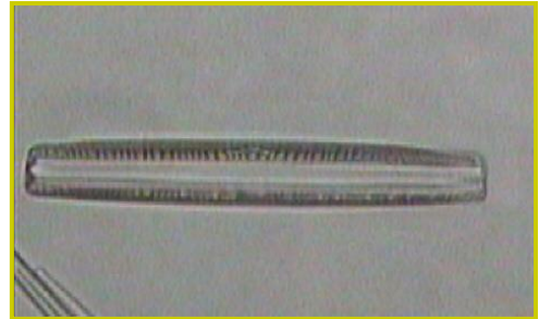
Diatoms sp
