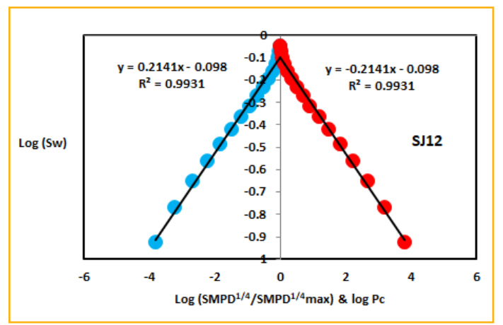
Figure 10: Log (SMPD 1/4 /SMPD 1/4max ) & log (α * h) versus log Sw for sample SJ12.
