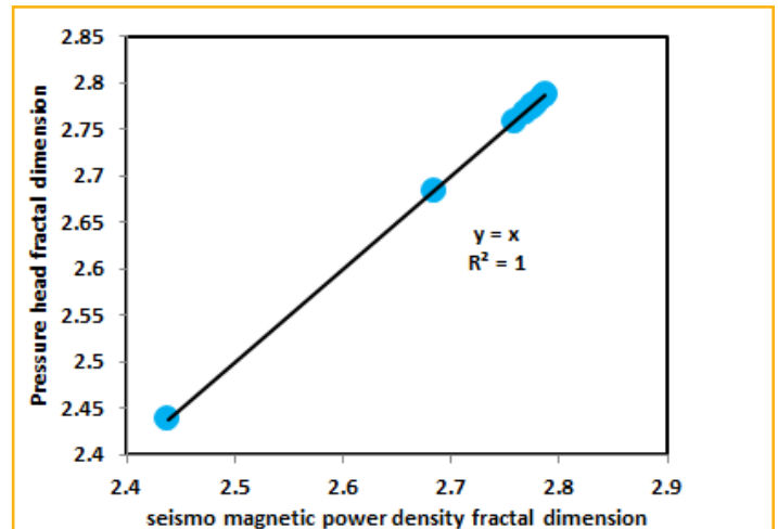
Figure 13: Seismo magnetic power density fractal dimension versus pressure head fractal dimension.
