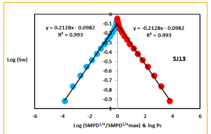
Figure 11: Log (SMPD 1/4 /SMPD 1/4max ) & log (α * h) versus log Sw for sample SJ13.
