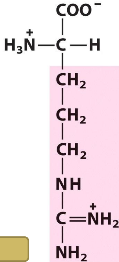
Arginine
