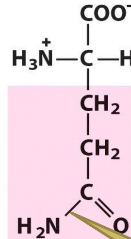
Glutamine
