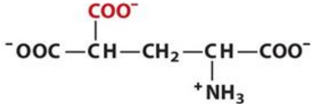
\gamma -Carboxyglutamate
