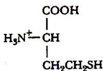
Homocysteine
