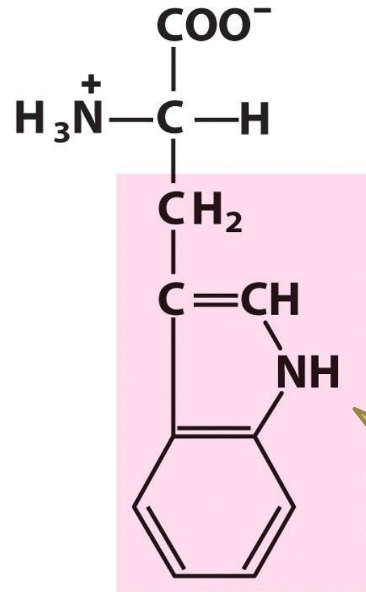
Tryptophan
