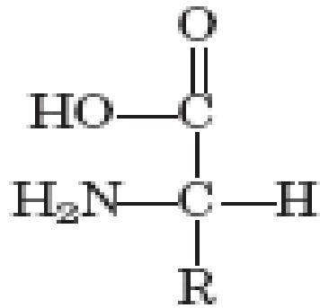
Nonionic form
