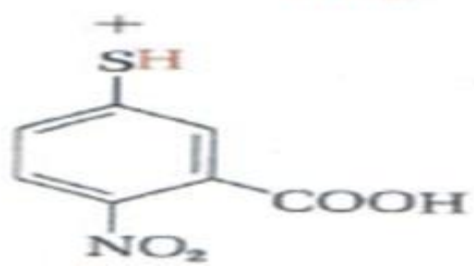
Thionitrobenzoic acid
