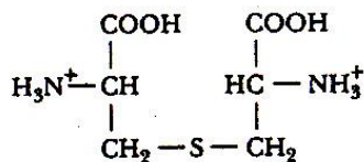
L-Lanthionine
