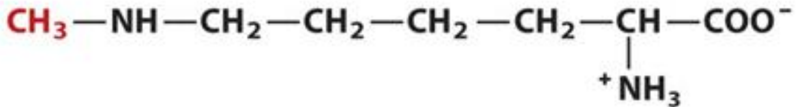
6-N-Methyllysine
