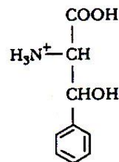
L-Phenylserine
