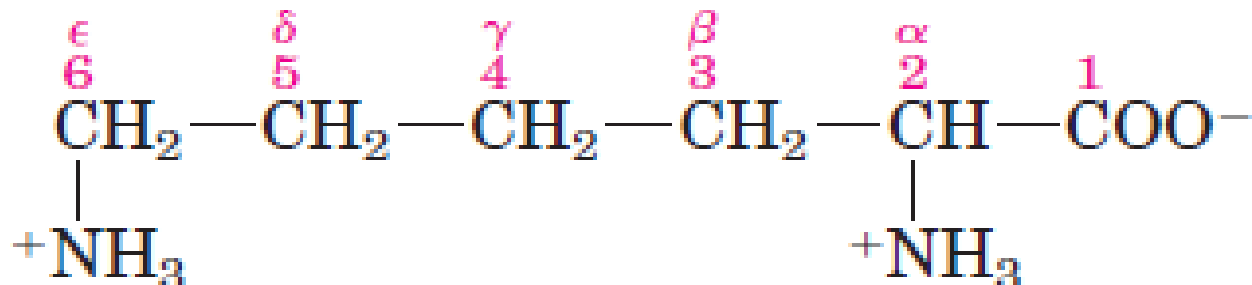
Lysine
