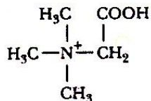
Betaine (N,N,N-trimethylglycine)
