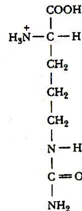
Citrulline
