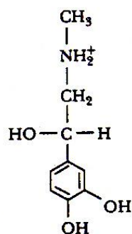
Epinephrine
