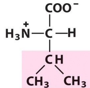
Valine
