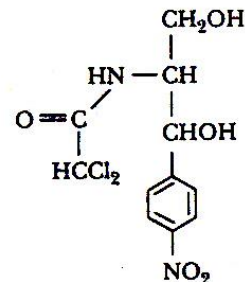
L-Chloramphenicol
