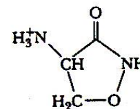
Cycloserine
