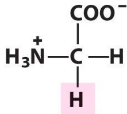
Glycine
