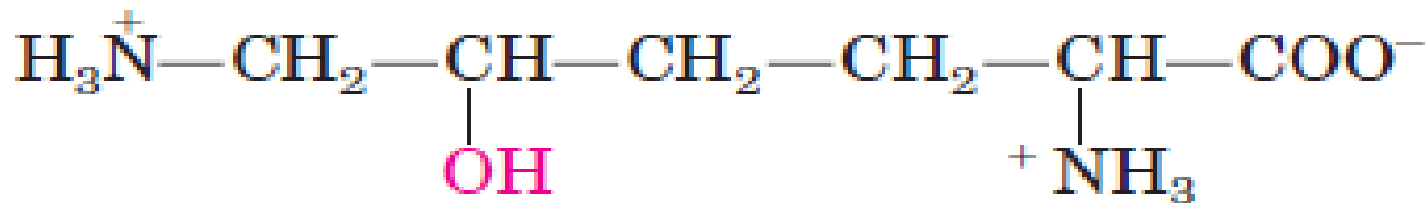
5-Hydroxylysine
