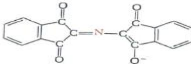
Purple pigment
