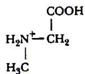
Sarcosine (N-methylglycine)
