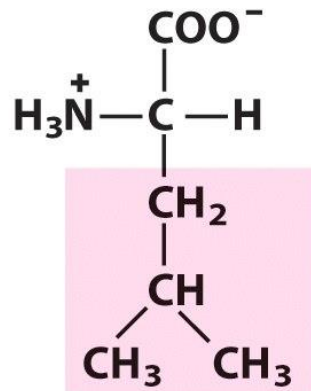
Alanine
