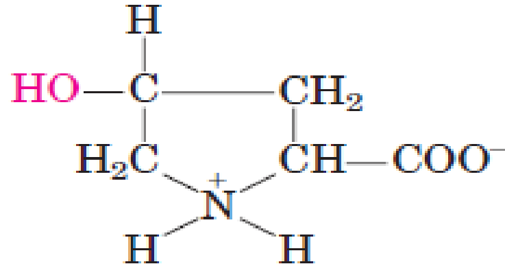
4-Hydroxyproline
