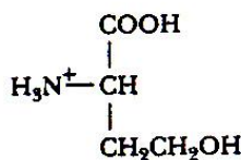
Homoserine
