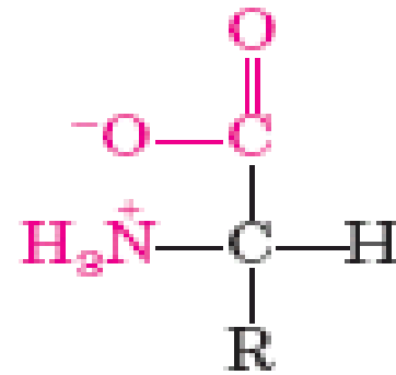
Zwitterionic form
