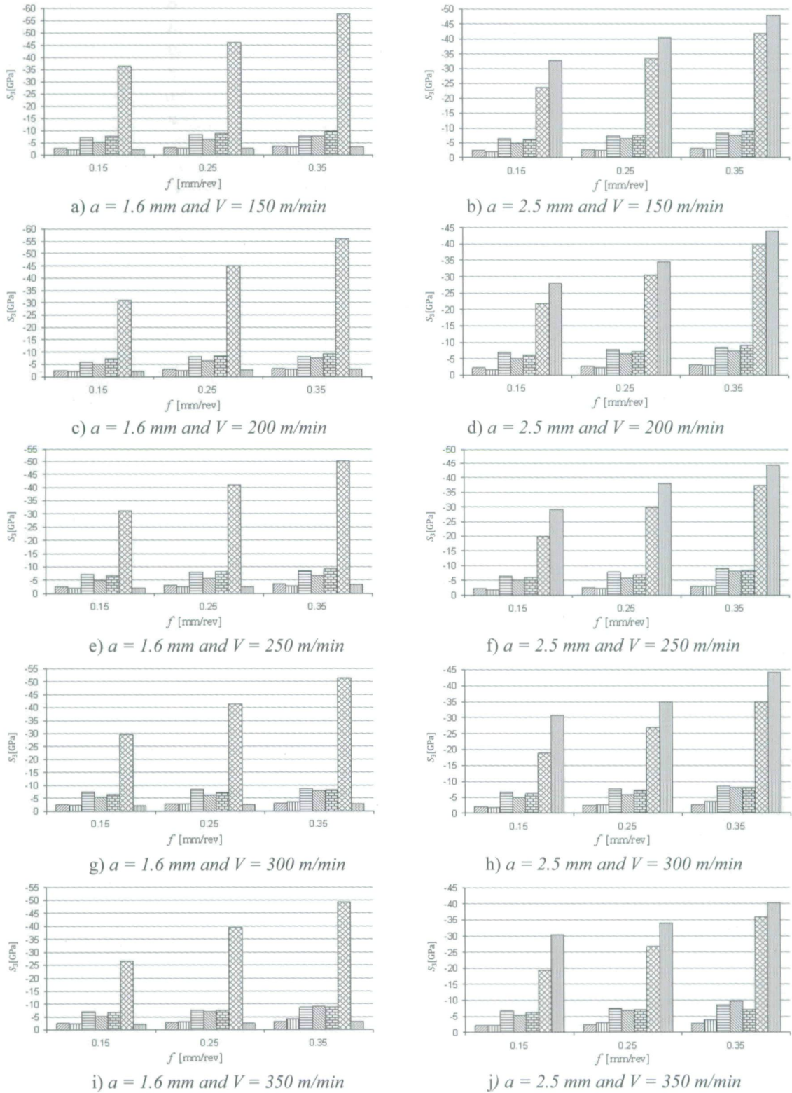
Fig. 4. Variation of minimum principal stress ( S_3 ) depending on chip breaker form
