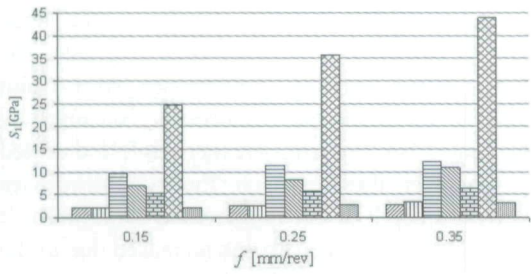
g) a = 1.6 \text{ mm} and V = 300 \text{ m/min}
