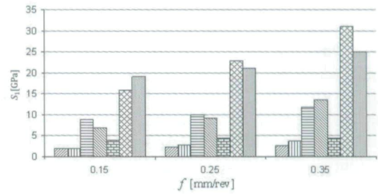
j) a = 2.5 \text{ mm} and V = 350 \text{ m/min}
