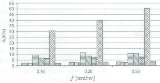
a) a = 1.6 \text{ mm} and V = 150 \text{ m/min}
