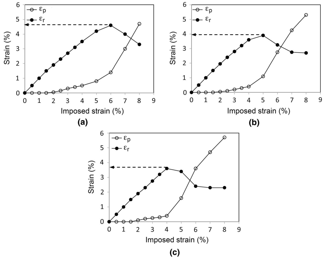
Fig. 5—Evolutions of the superelastic recovery strain, \epsilon_r , and the residual plastic strain, \epsilon_p as the function of the imposed strain during loading–unloading cycles for the Ti-23Hf-3Mo-Sn alloy specimens solution treated at 1073 K for 0.3 ks (a), 0.6 ks (b) and 3.6 ks (c).
