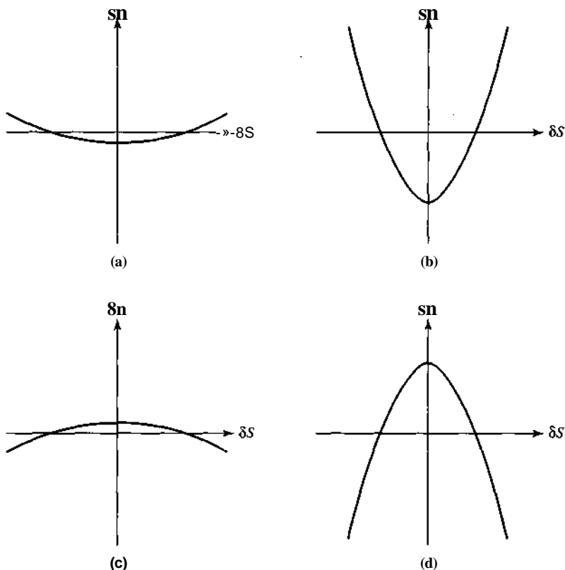
Figure 14.8 Alternative relationships between ST_i and \delta S for a delta-neutral portfolio: (a) slightly positive gamma, (b) large positive gamma, (c) slightly negative gamma, and (d) large negative gamma
