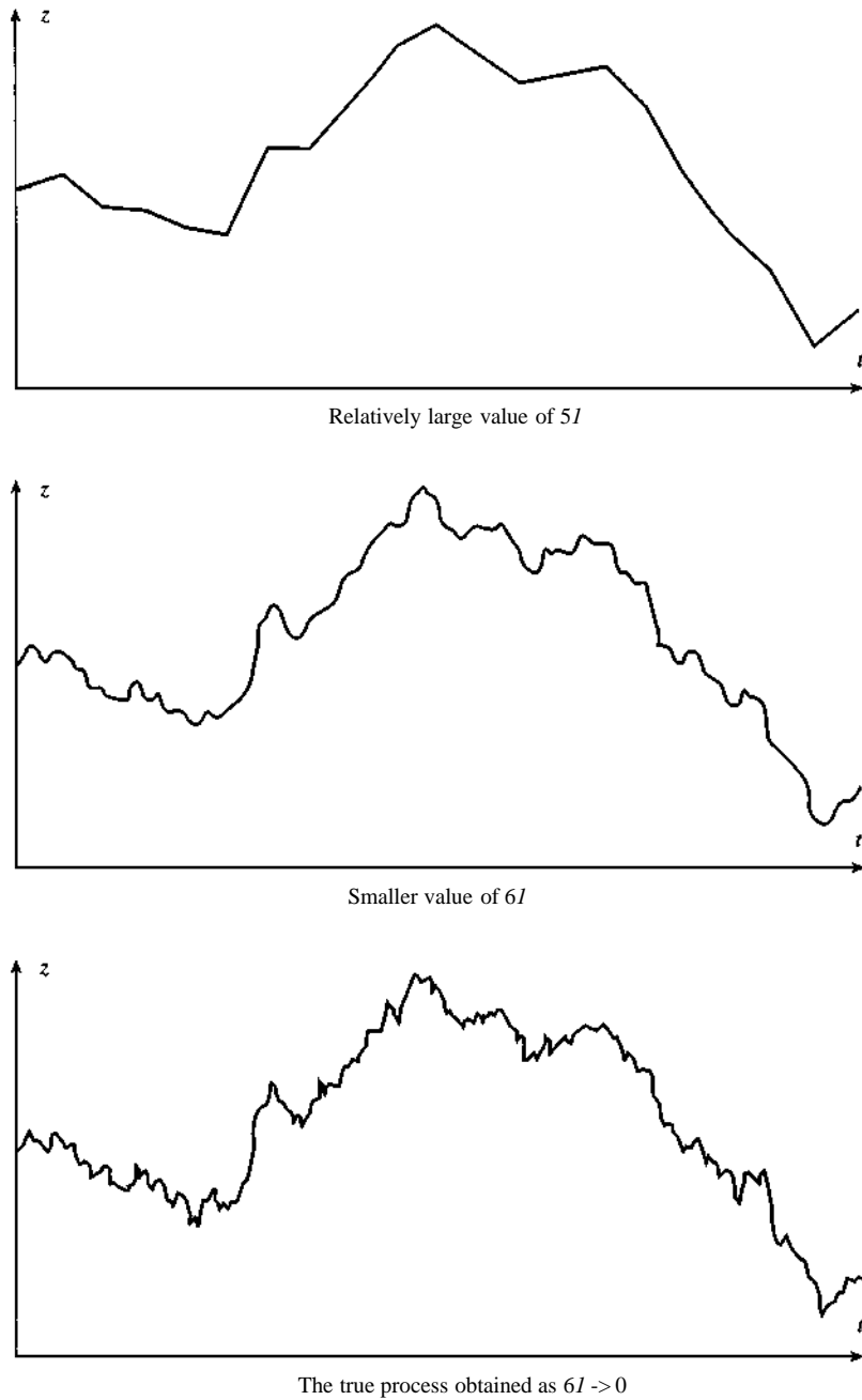
Figure 11.1 How a Wiener process is obtained when St \rightarrow 0 in equation (11.1)
