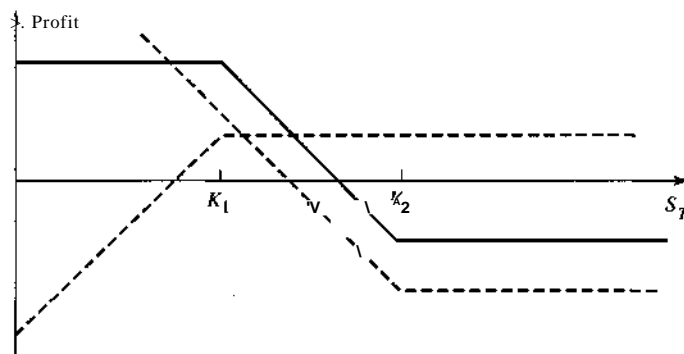
Figure 9.5 Bear spread created using put options
