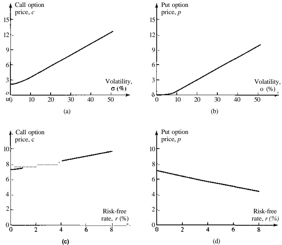
Figure 8.2 Effect of changes in volatility and risk-free interest rate on option prices when S_o = 50 , K = 50 , r = 5\% , a = 30\% , and T = 1 .
