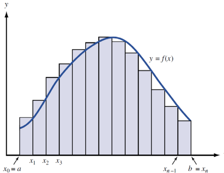
FIGURE 1 Relation of Area and Definite Integral
