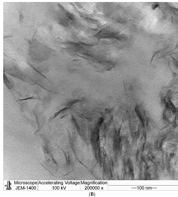
Figure 4. TEM images of (A) free 1% PCN at high magnification and (B) Free 3% PCN at high magnification.
