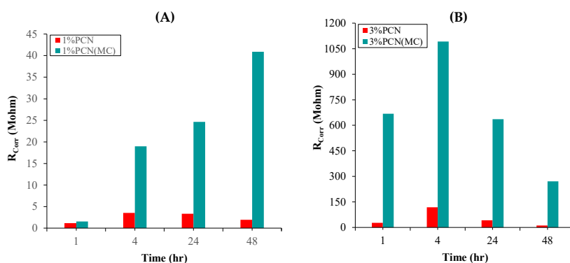
Figure 8. Corrosion resistance R_{\text{Corr}} ( \text{M}\Omega ) vs. time at 1, 4, 24 and 48 h for (A) Free and impregnated 1%PCNs, and (B) Free and impregnated 3%PCNs immersed in 3.5 wt.% NaCl at room temperature 20 \pm 0.5 \text{ }^\circ\text{C} .
